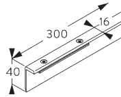
SG 6512 Connection bridge
