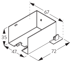
SG 11897 Recess mask
