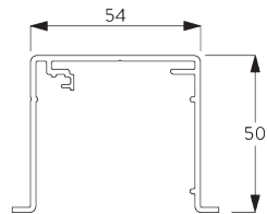
SG 11865 Recess profile
